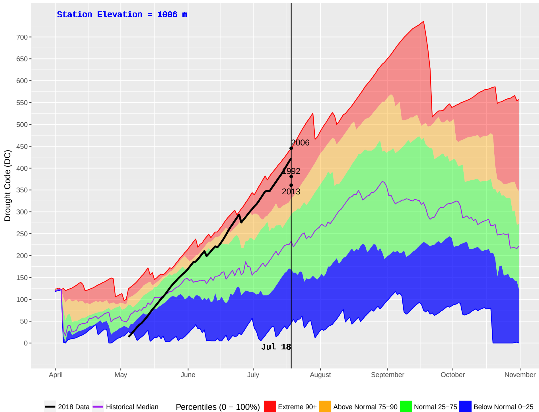
BENSON (228) : Historical (1987–2016) and Current (2018) Daily Drought Code (DC)
