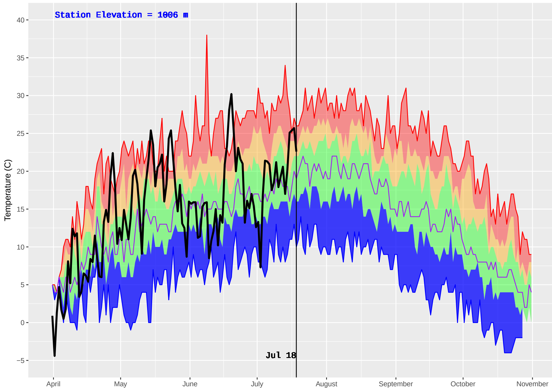
BENSON (228) : Historical (1987–2016) and Current (2018) Daily Temperature
